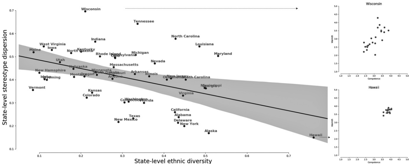
Fig. 2. Inverse linear relationship between ethnic diversity and stereotype dispersion in 50 states in the United States. Note that analysis unit is state in the United States, n = 50 . The x axis indicates contextual ethnic diversity from the most homogeneous (left) to the most diverse (right). The y axis indicates stereotype dispersion from the least dispersed (bottom) to the most dispersed (top) maps of warmth-by-competence space. Each dot represents one state; see Results for statistics. We depict the extreme cases (i.e., Wisconsin and Hawaii) as clearly illustrating the range of stereotype dispersion. See Results for statistics, and see SI Appendix for maps for each state.
