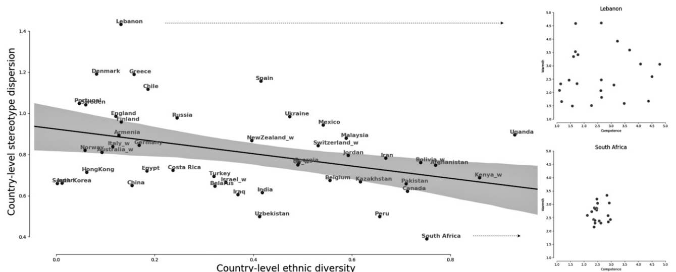
Fig. 1. Inverse linear relationship between ethnic diversity and stereotype dispersion in 46 nations. Note that analysis unit is country or region, n = 46 . The x axis indicates contextual ethnic diversity from the most homogeneous (left) to the most diverse (right). The y axis indicates stereotype dispersion from the least dispersed (bottom) to the most dispersed (top) maps in warmth-by-competence space. Each dot represents one country; see Results for statistics. We depict the extreme cases (i.e., Lebanon and South Africa) as clearly illustrating the range of stereotype dispersion. See Results for statistics, and see SI Appendix for maps for each country.
